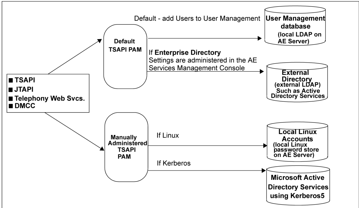
Figure 24: AE Services client authentication -- additional PAM management
