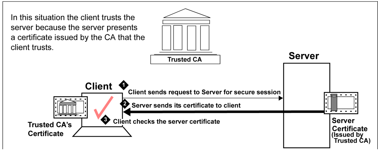
Figure 20: Server authentication
