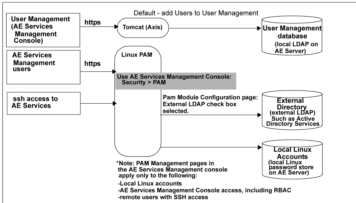
Figure 17: AE Services and ssh authentication methods
