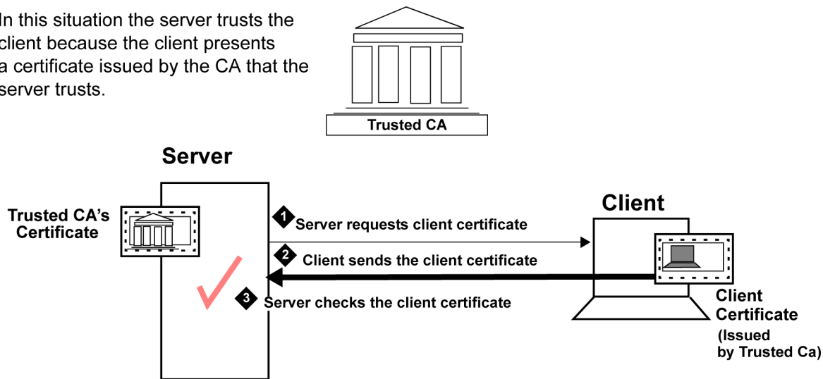
Figure 21: Client Authentication
