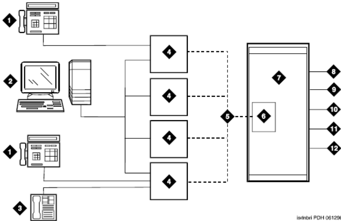
Figure 6: ISDN—BRI Personal Computer interface configuration (Group 2)
