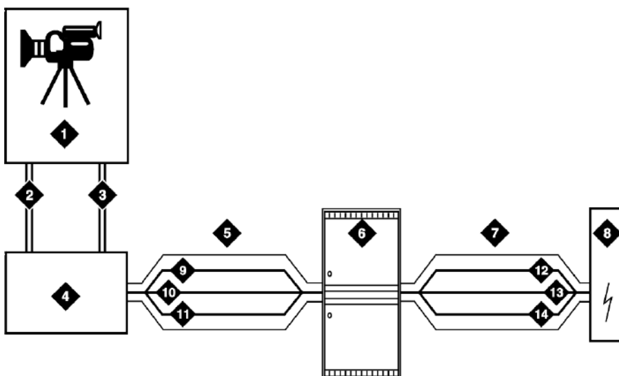
Figure 7: Typical video broadband application
