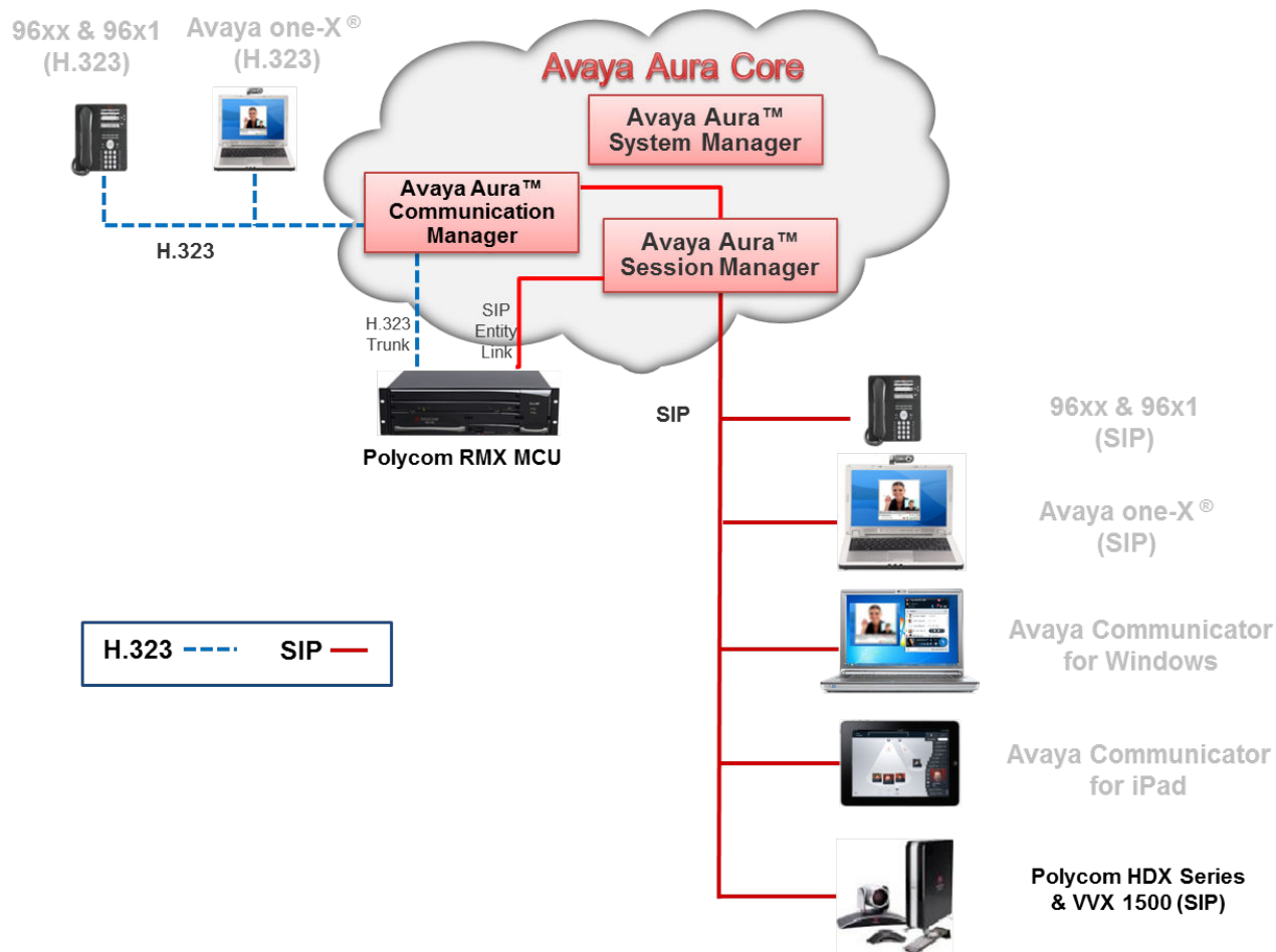
Figure 7: Avaya Aura® and SIP-based Polycom endpoints interoperability
