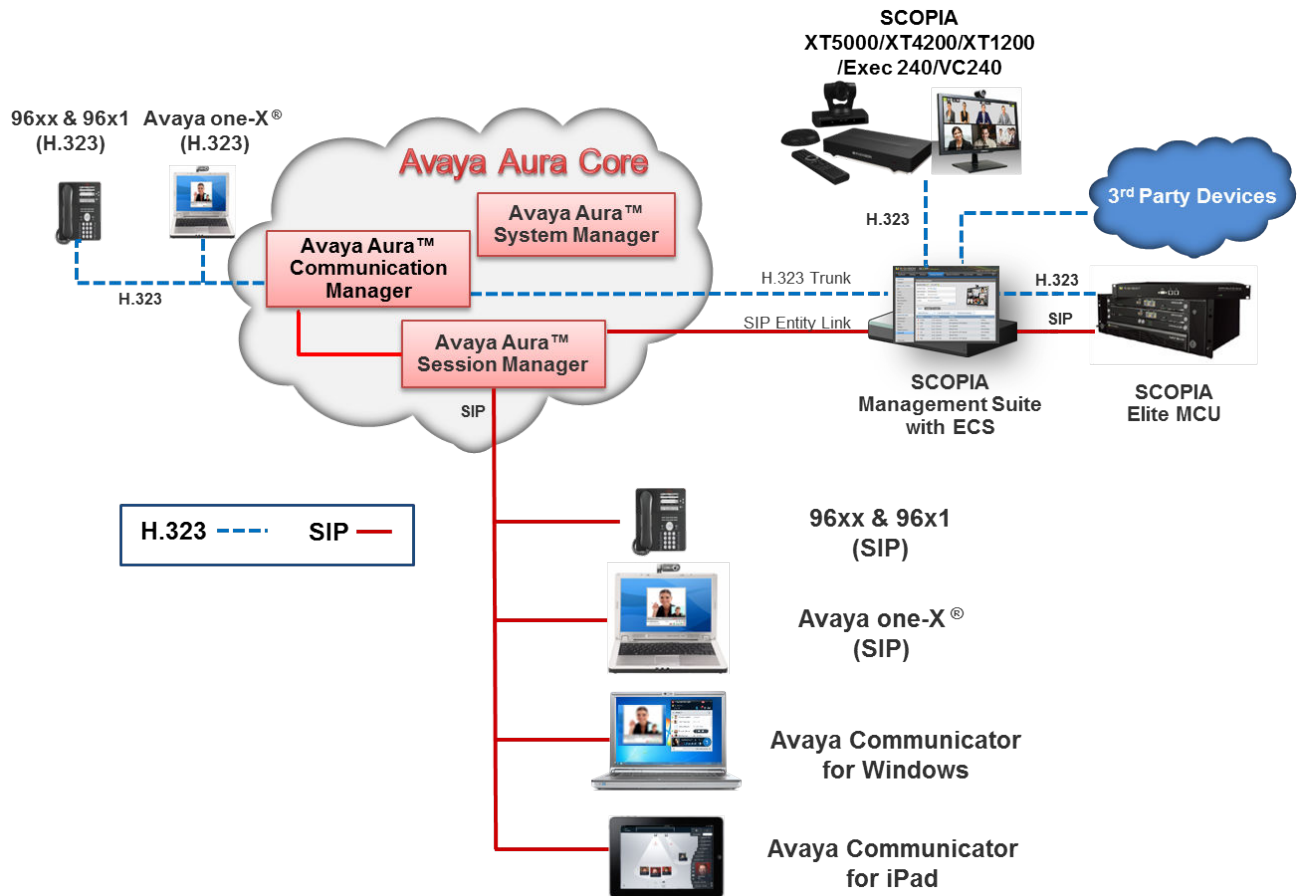
Figure 5: Avaya Aura® and Scopia interoperability with third-party endpoints
