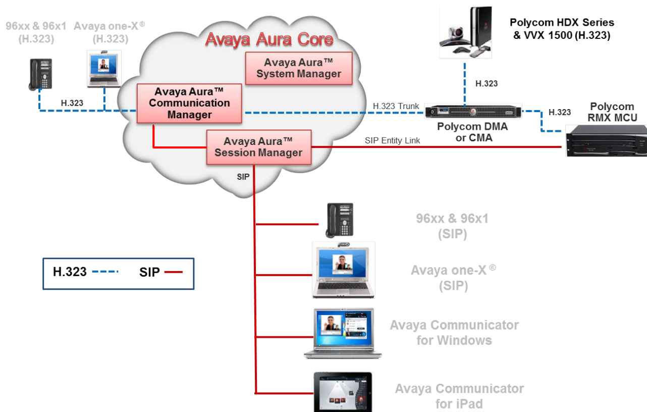
Figure 8: Avaya Aura® and Polycom interoperability
