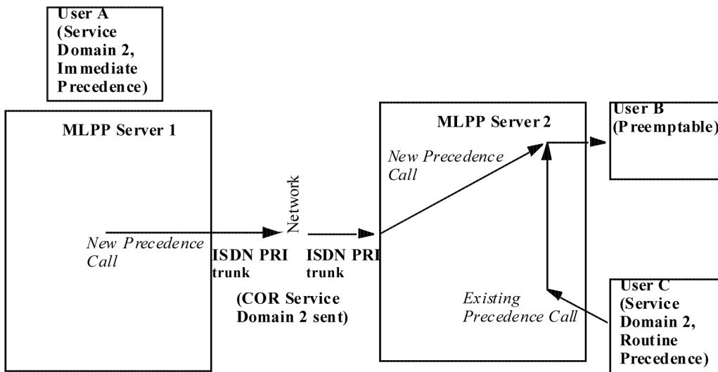
Figure 24: Precedence calls to destinations over ISDN-PRI trunks
