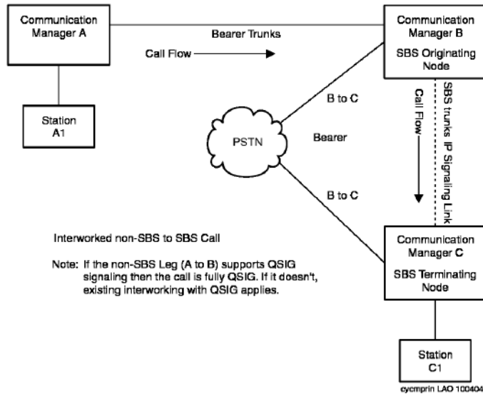
Figure 30: PRI Non-SBS to SBS Call Connections
