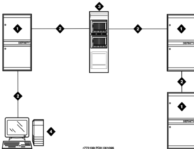
Figure 17: ISDN network configuration
