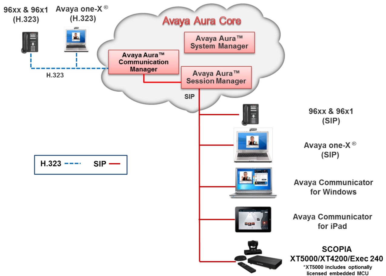
Figure 3: Avaya Aura® Conferencing without external gatekeepers or MCUs configuration
