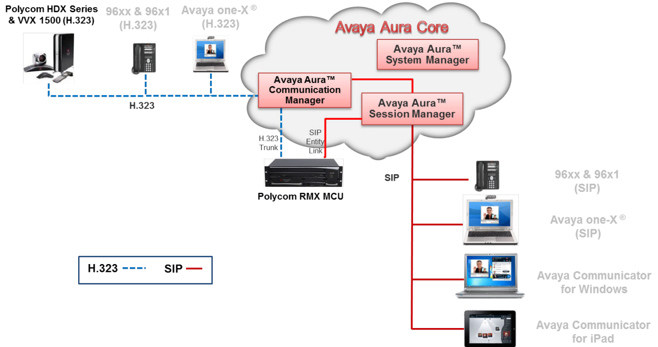
Figure 6: Avaya Aura® with H.323-based Polycom endpoints through Communication Manager and Polycom RMX.
