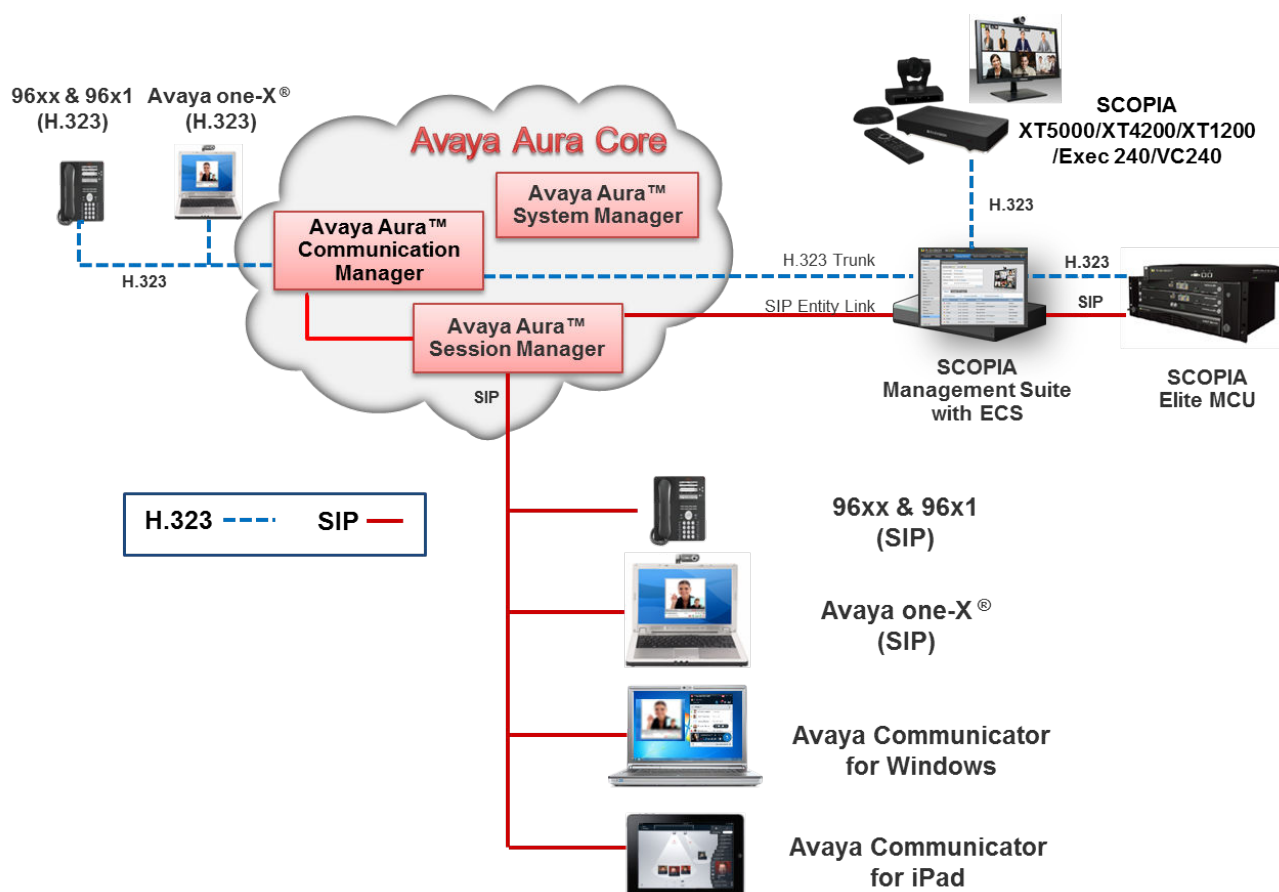
Figure 4: Avaya Aura® and Scopia interoperability
