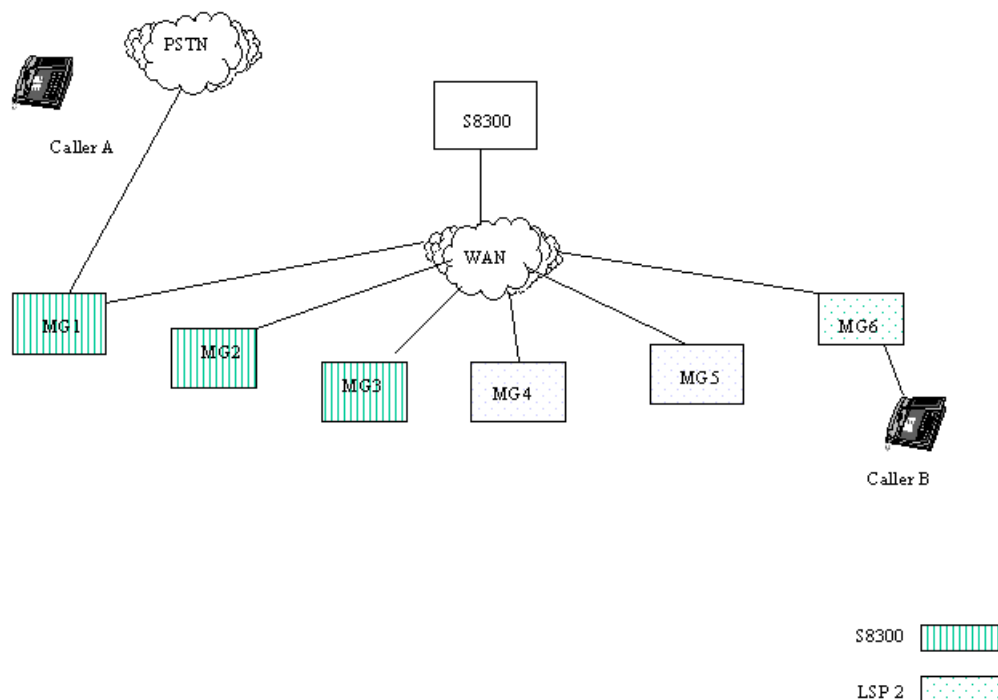
Figure 11: Trunk-to-Station call between main server and gateway during network outage
