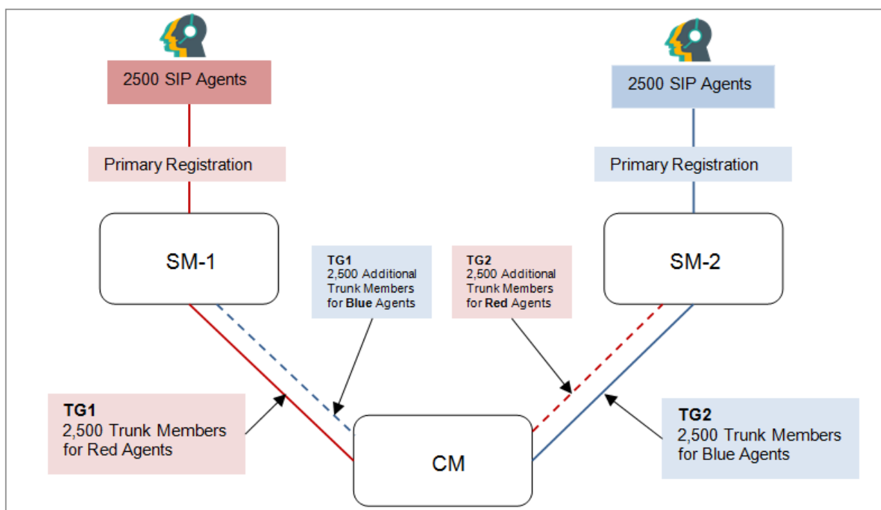
Figure 32: Scenario 2 of trunk consumption due to redundancy
