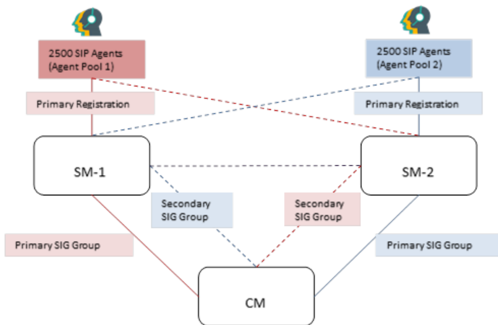
Figure 31: Scenario 1 of trunk consumption due to redundancy
