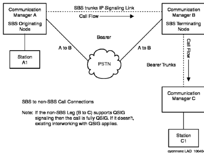
Figure 29: SBS to non-SBS QSIG Call Connections
