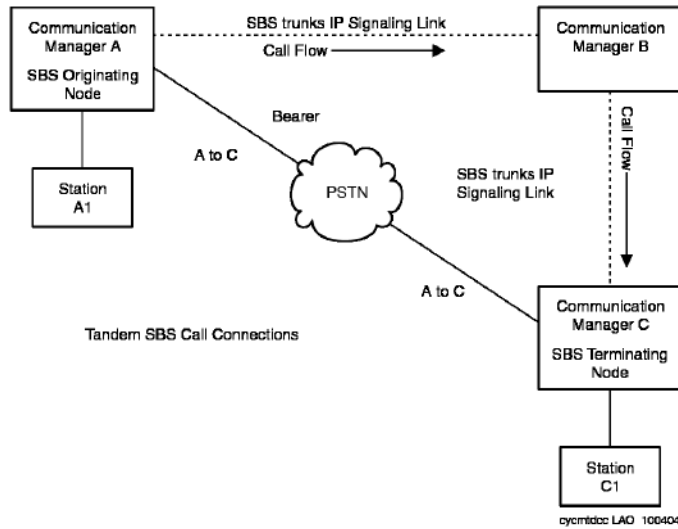
Figure 28: Tandem SBS Call Connections
