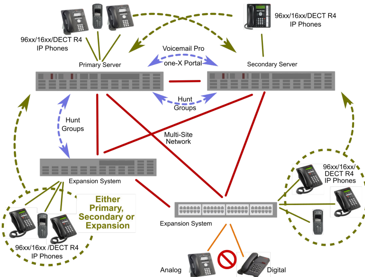
Figure 2: Resiliency Architecture
