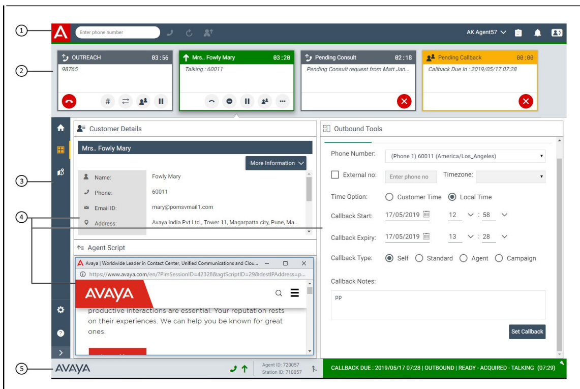
Figure 1: POM Workspaces user interface
